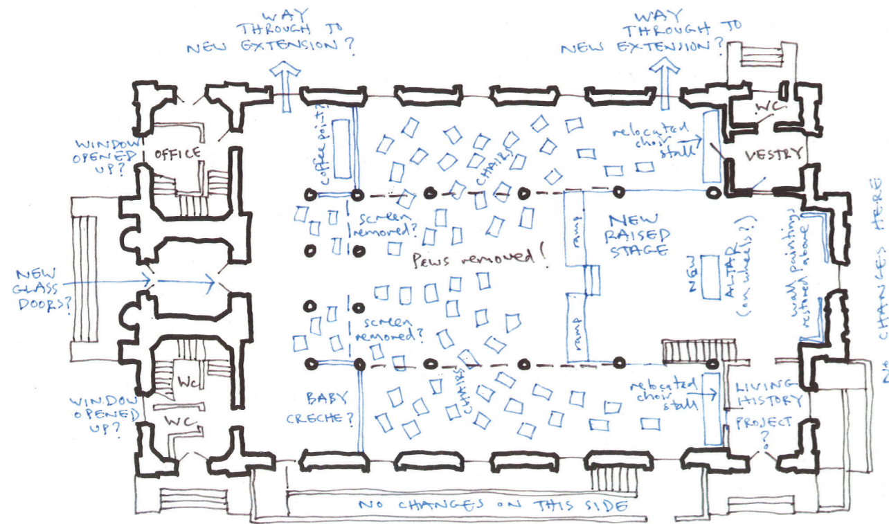
INITIAL SKETCH IDEAS FOR GROUND FLOOR OF EXISTING CHURCH
